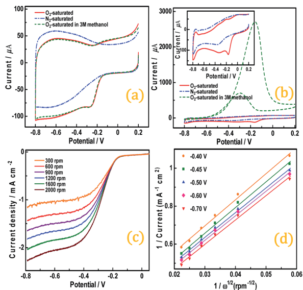
Fig. 4 (a and b) CVs of N-CD/graphene and commercial Pt/C on a GC electrode in O_2 -saturated 1 M KOH, N_2 -saturated 1 M KOH and O_2 -saturated 1 M KOH containing 3 M CH_3OH at a scan rate of 50\text{ mV s}^{-1} . The inset in (b) show amplified CVs of commercial Pt/C in O_2 -saturated 1 M KOH, N_2 -saturated 1 M KOH. (c) Rotating disk electrode (RDE) curves for N-CD/graphene in O_2 -saturated 1 M KOH with various rotation rates at a scan rate of 10\text{ mV s}^{-1} . (d) The Koutecky–Levich plots derived from the RDE measurements.
