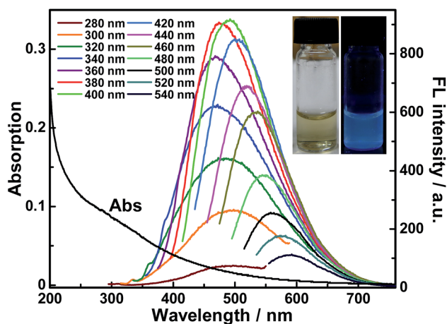
Fig. 3 UV-Vis absorption and PL spectra (recorded for progressively longer excitation wavelengths in 20 nm increments) of the obtained N-CDs. Inset: photograph of the obtained N-CDs under illumination of white light (left) and UV (365 nm) light (right).
