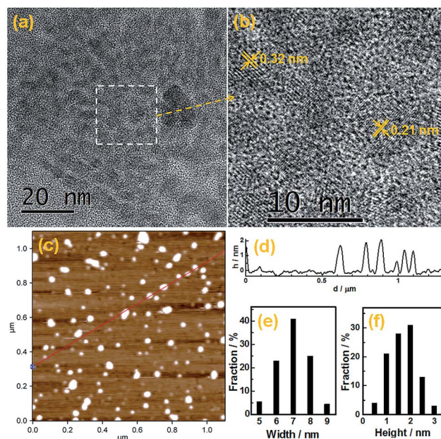
Fig. 1 (a) and (b) are TEM and HRTEM images of the N-CDs. (c) AFM image of the N-CDs. (d) Height profile along the line in (c). (e) and (f) show the width and height distributions of the N-CDs.
